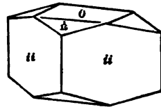
Phenixville.
